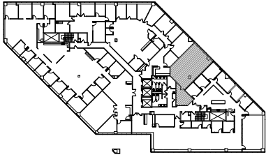
3RD FLOOR KEY PLAN
